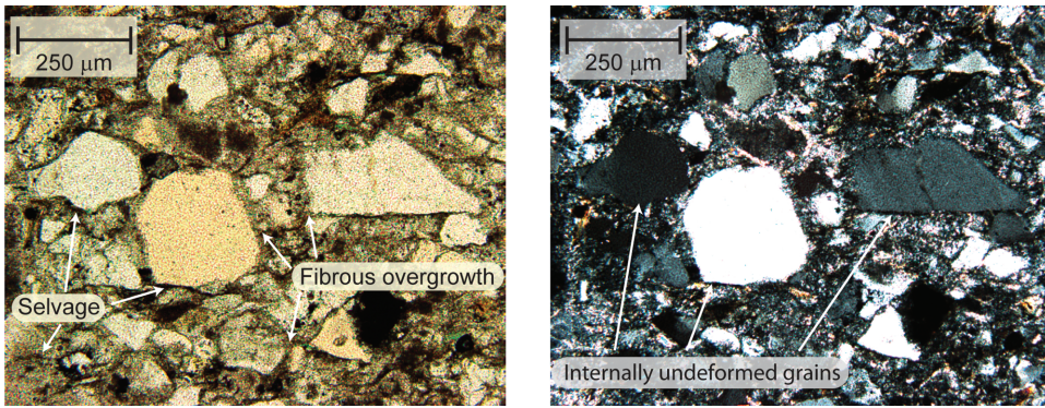
Fig. 7. Plane and polarized light images from sample 000303-4 illustrating the microstructures of the Ottago Schist rocks.
