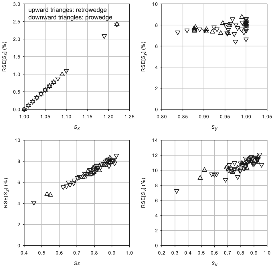
Fig. 12. Plots showing relative standard errors for principal stretch values, determined through bootstrap analysis (Efron and Tibshirani, 1994).
