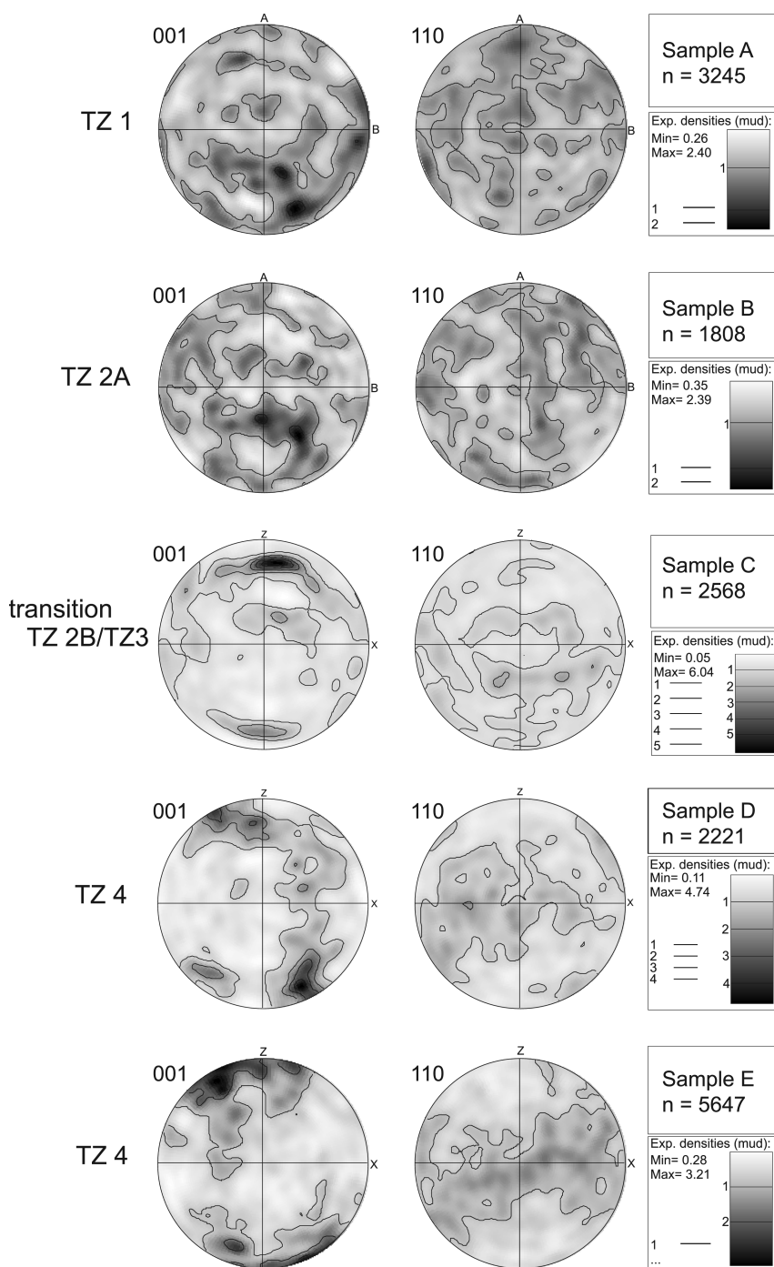
Fig. 9. Lower hemisphere, equal area stereonet showing electron back-scatter diffraction orientation data for 001 and 110 lattice directions in quartz from five samples of the Otago Schist (locations shown on fig. 5). Lower textural zone samples (TZ 1 and TZ 2A) show no lattice preferred orientation (LPO), indicating that dislocation glide was not active, which is consistent with other evidence indicating that grain-boundary pressure solution was the dominant deformation mechanism for these textural zones. In contrast, rocks from TZ 2B and higher do show quartz LPO, indicating that intracrystalline deformation has occurred.
